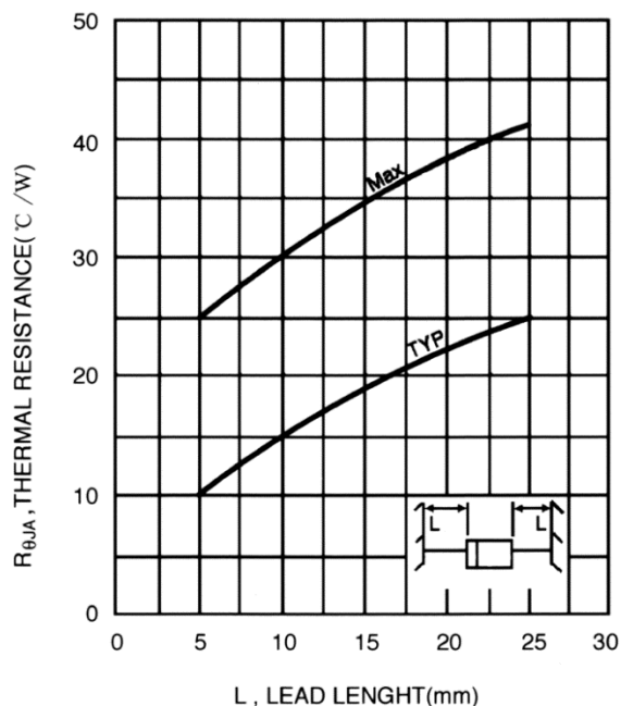
FIG. 4 – TYPICAL THERMAL RESISTANCE
