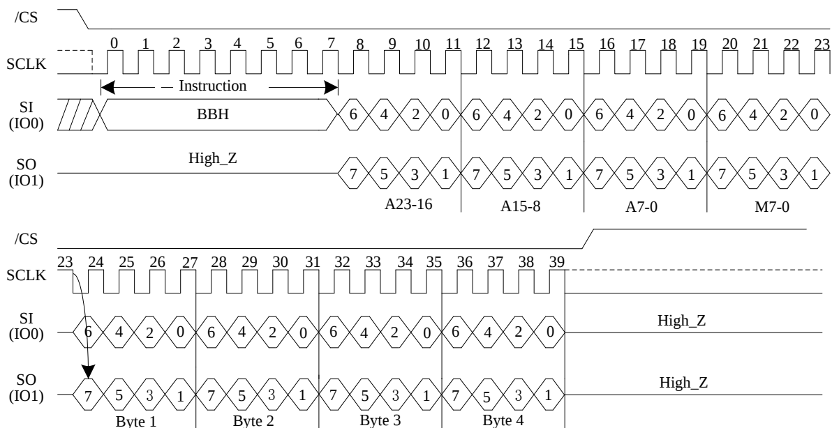
Figure 14. Dual I/O Fast Read Sequence Diagram (Initial command or previous (M5-4) \neq (1,0))
