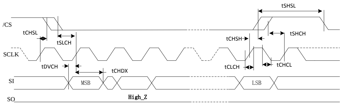
Figure 47. Output Timing
