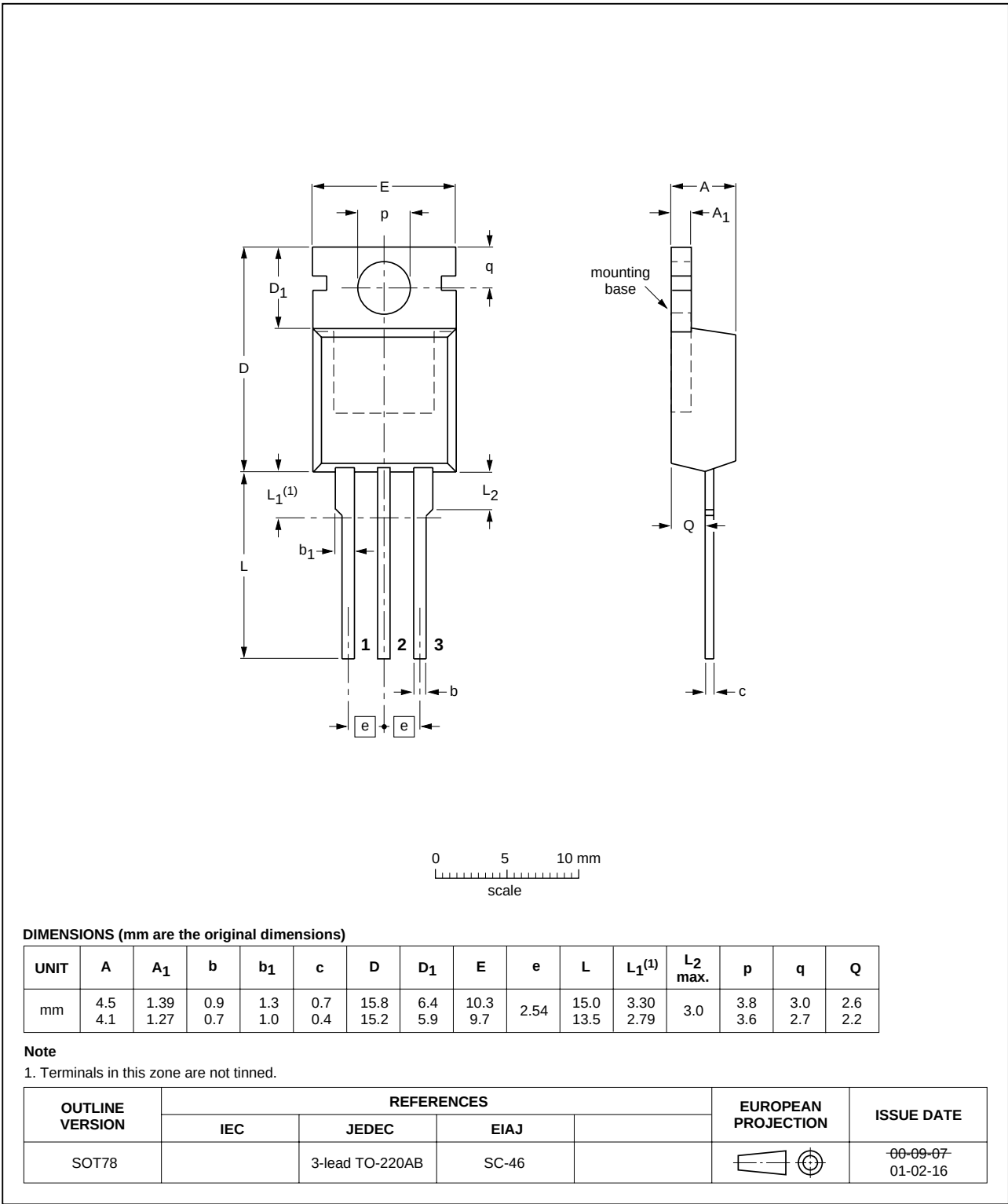
Fig 16. SOT78 (TO-220AB).
