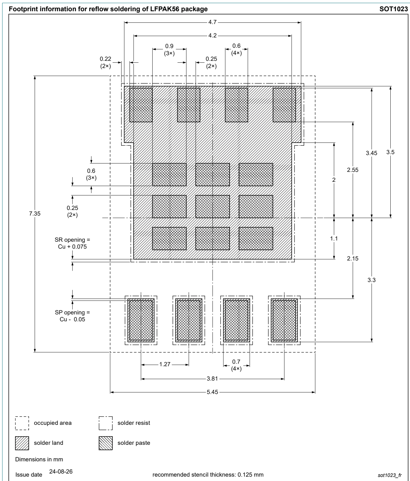
Fig. 18. Reflow soldering footprint for LPAK56E; Power-SO8 (SOT1023)
