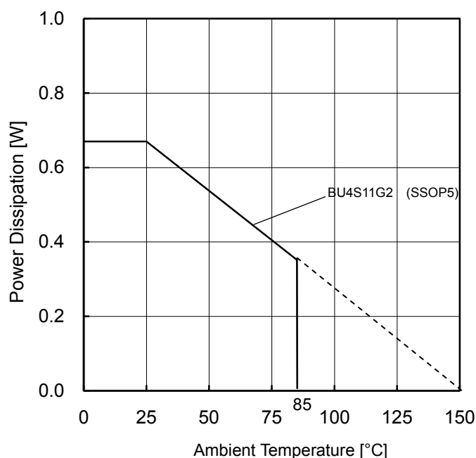
Figure 12. Derating Curve
