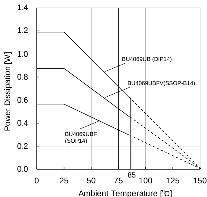
Figure 11. Derating Curve
