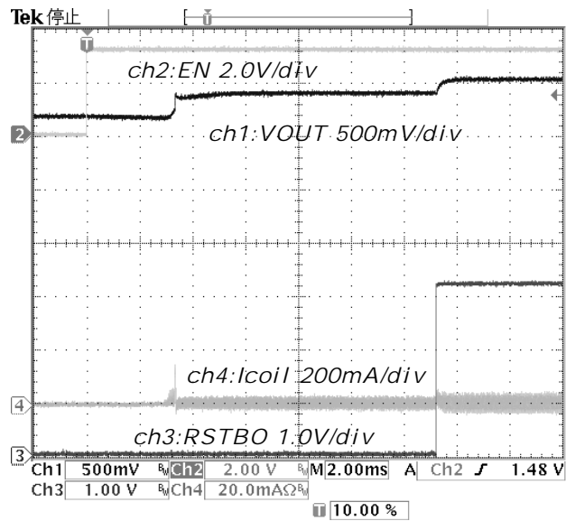
Figure 24. RISE [EN : OFF=>ON] PWM VIN=3.3V Io=0mA
