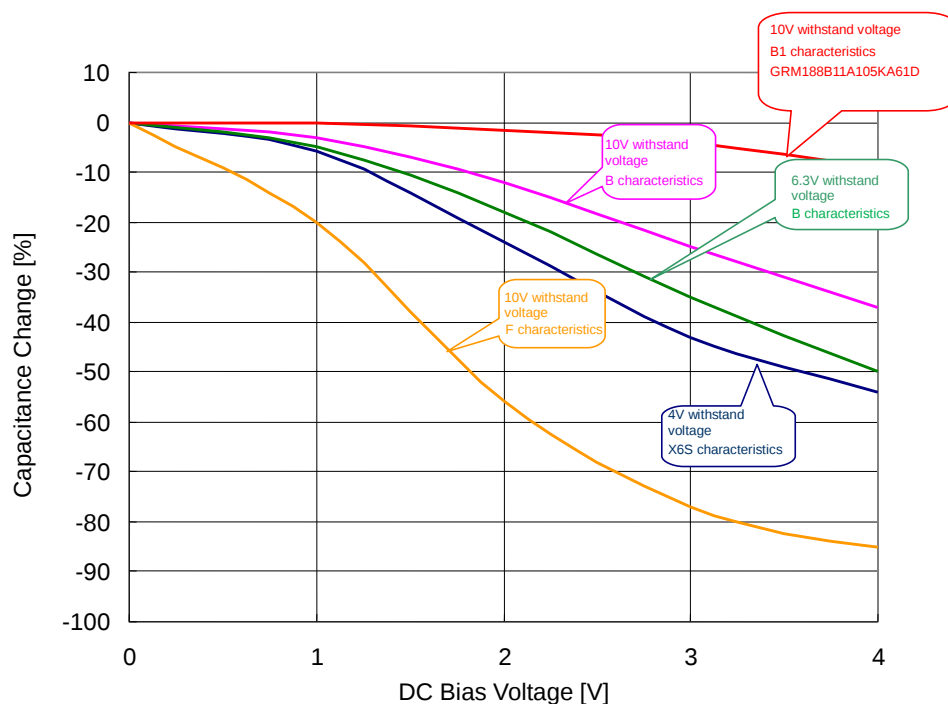
Figure 31. Capacity-bias characteristics
