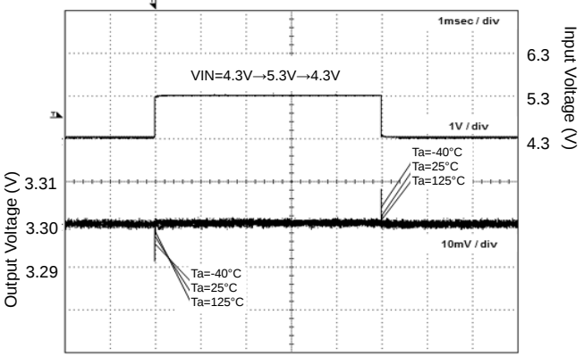
Figure 28. VIN Response
