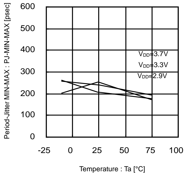
Figure 42. Period-Jitter MIN-MAX vs Temperature (14.3MHz)
