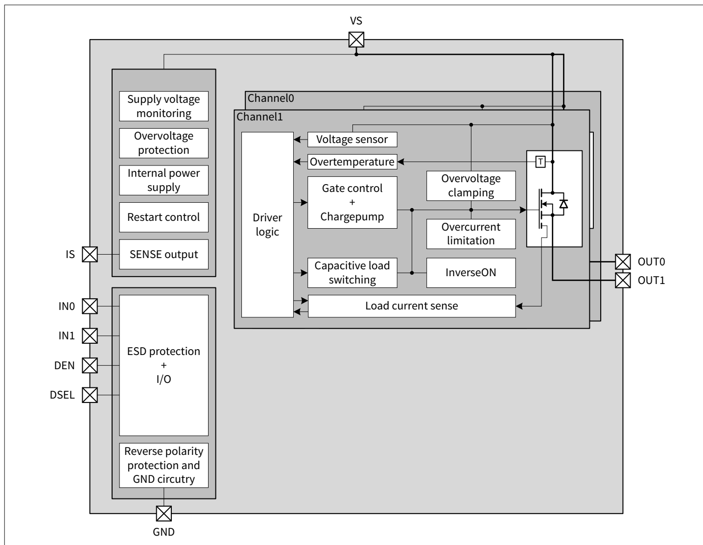
Figure 2 Block diagram of BTS7050-2EPL
