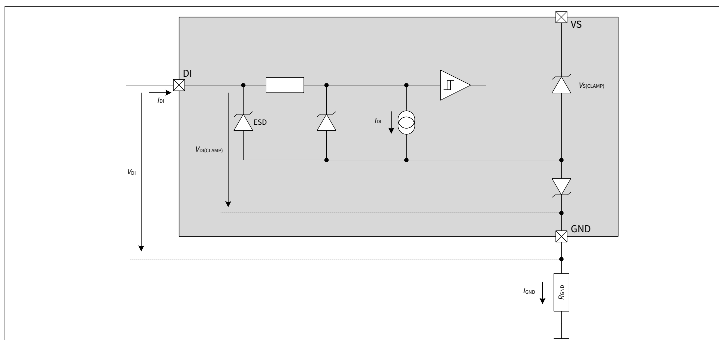
Figure 11 Input circuitry
