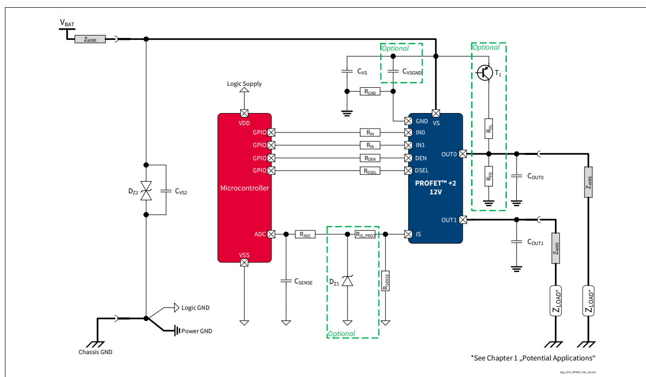
Figure 1 BTS7030-2EPA Application Diagram. Further information in Chapter 10
