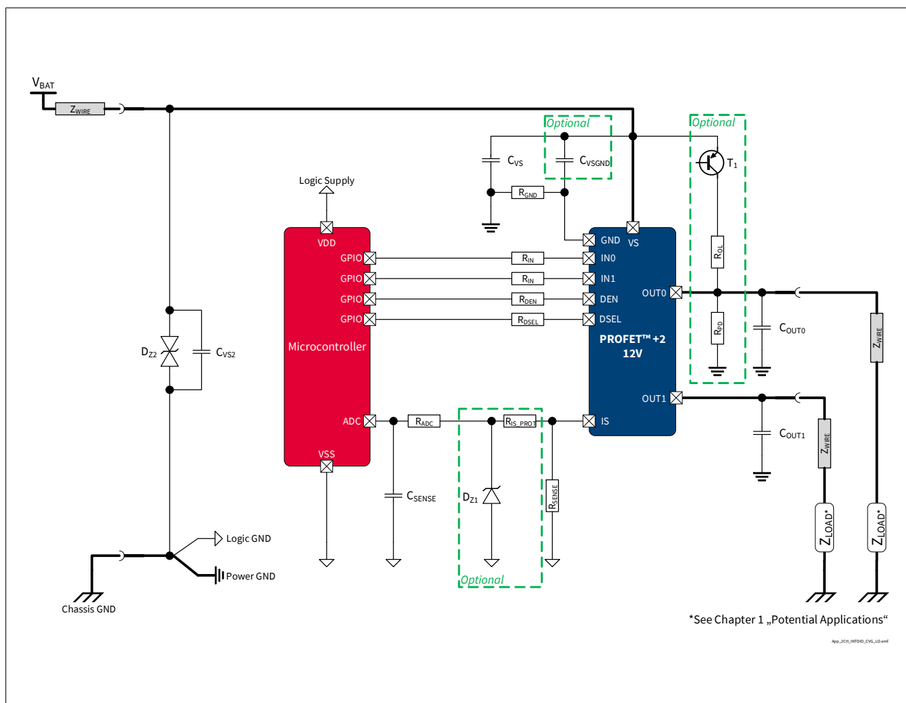
Figure 43 BTS7012-2EPG Application Diagram
