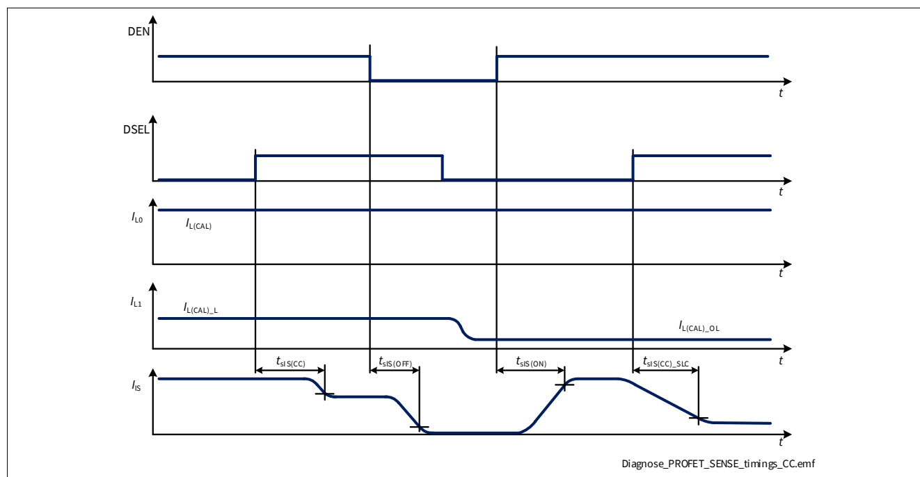
Figure 42 SENSE Settling Timing - Channel Change
