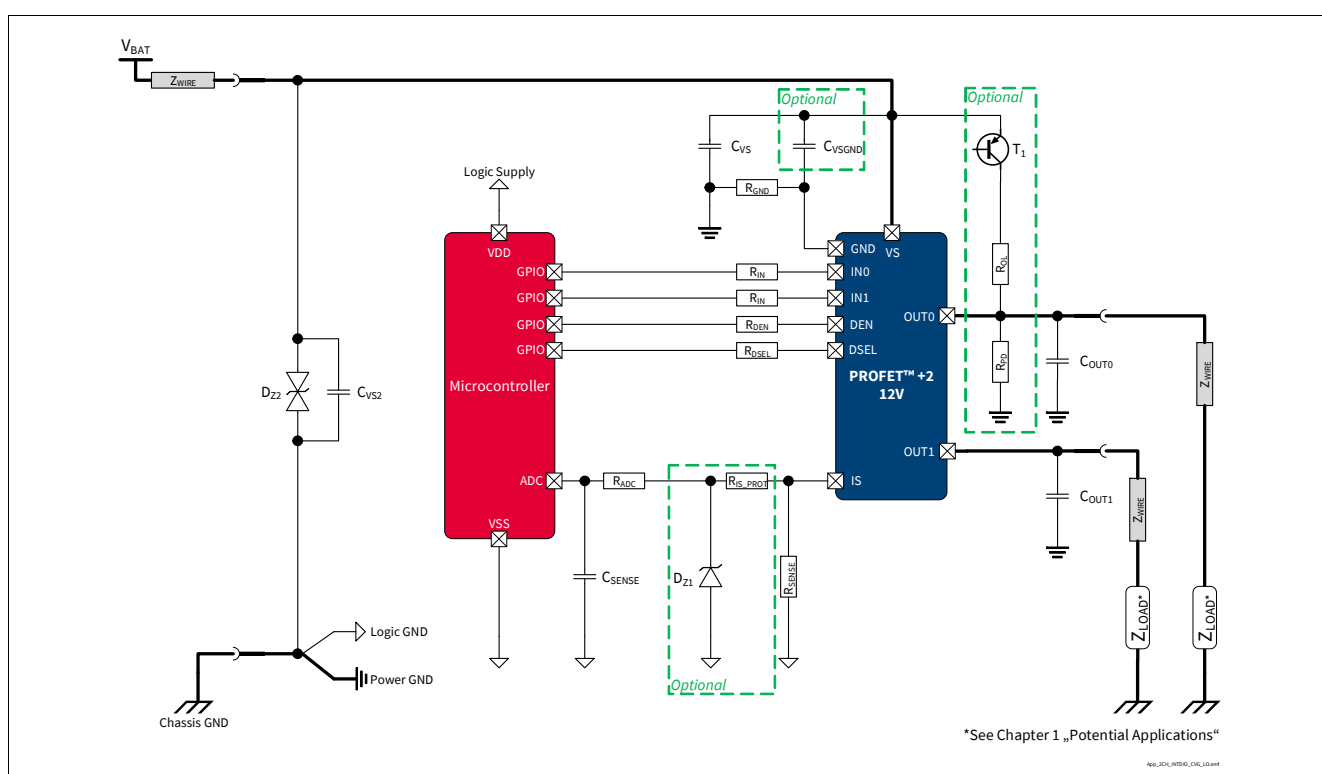
Figure 1 BTS7012-2EPG Application Diagram. Further information in Chapter 10
