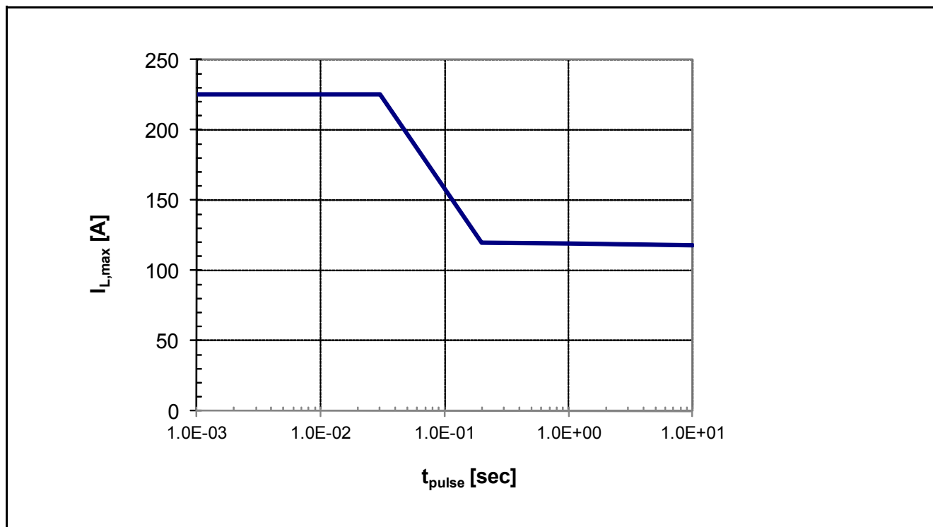
Figure 4 Maximum Single Pulse Current vs. Pulse Time, T_J \leq 150^\circ\text{C} , T_{amb} = 85^\circ\text{C}
