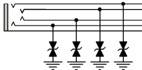
Earphone Jacket
