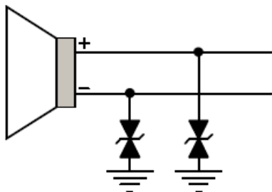
Speaker
