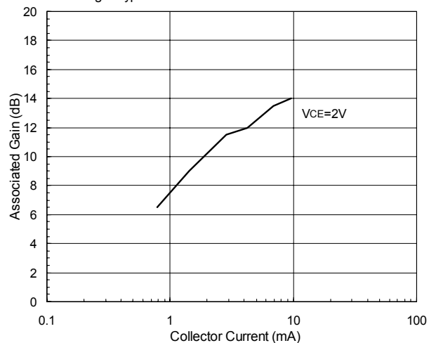
Fig.6 Typical Associated Gain & Collector Current
