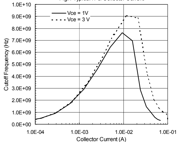
Fig.4 Typical f_T & Collector Current
