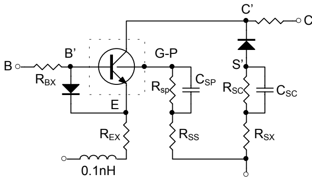
Transistor Chip Equivalent Circuit
