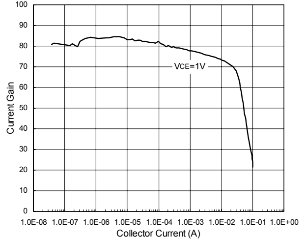
Fig.2 Typical Forward Current Gain & Collector Current
