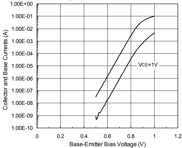
Fig.1 Typical Forward Gummel Plot
