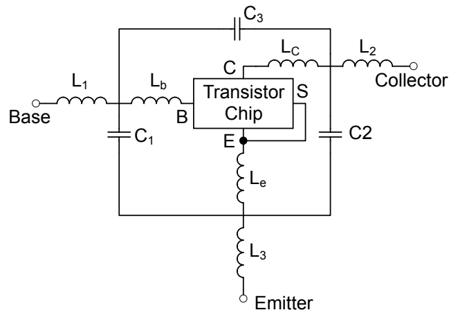
Package Equivalent Circuit
