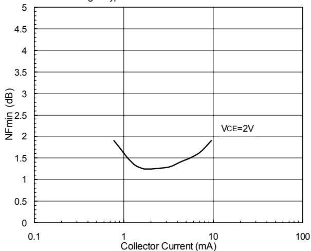
Fig.5 Typical NFmin & Collector Current
