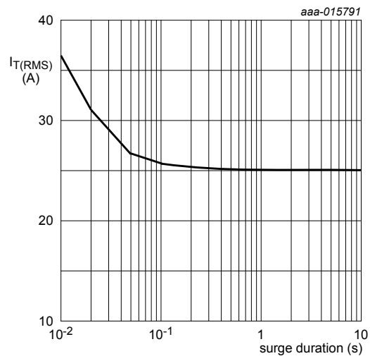
Fig. 2. RMS on-state current as a function of surge duration; maximum values f = 50 \text{ Hz}; T_{mb} = 100 \text{ °C}
