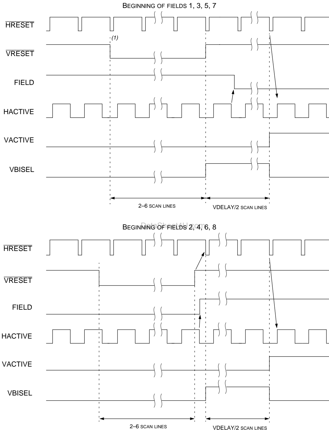
Figure 40. Video Timing in SPI Output Mode
