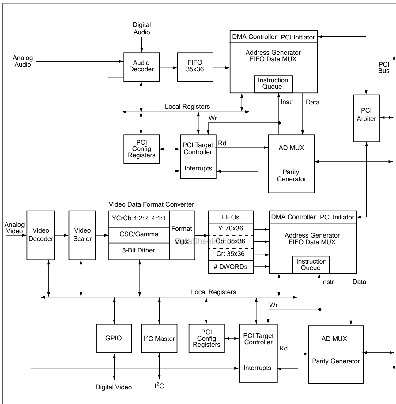
Figure 1. Bt879 Detailed Block Diagram
