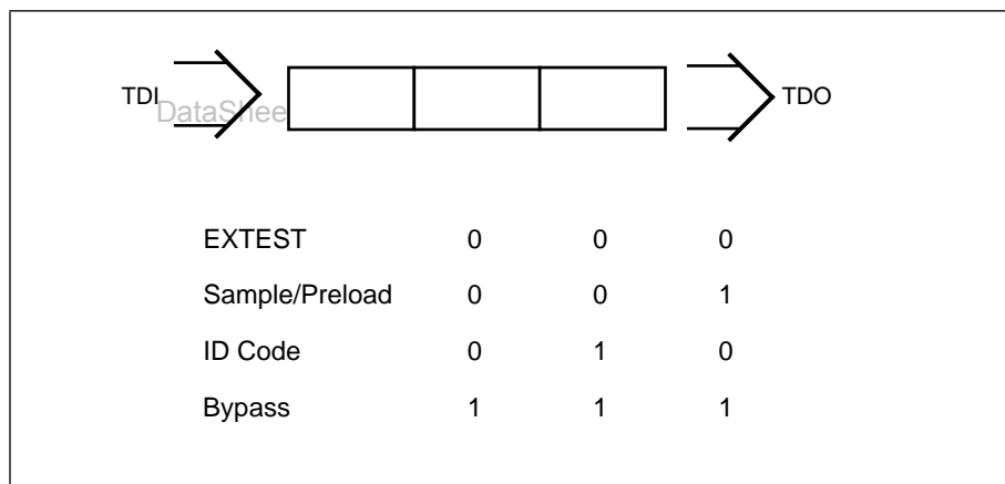
Figure 45. Instruction Register
