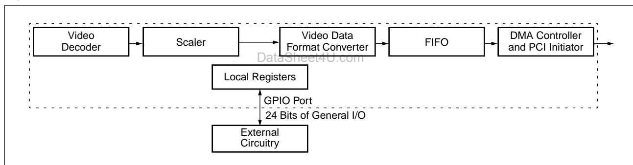
Figure 35. GPIO Normal Mode
