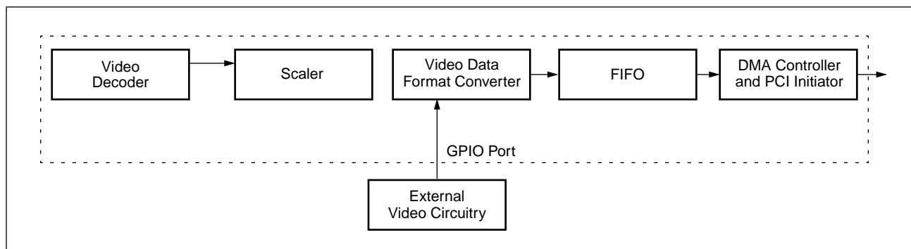
Figure 36. GPIO SPI Input Mode
