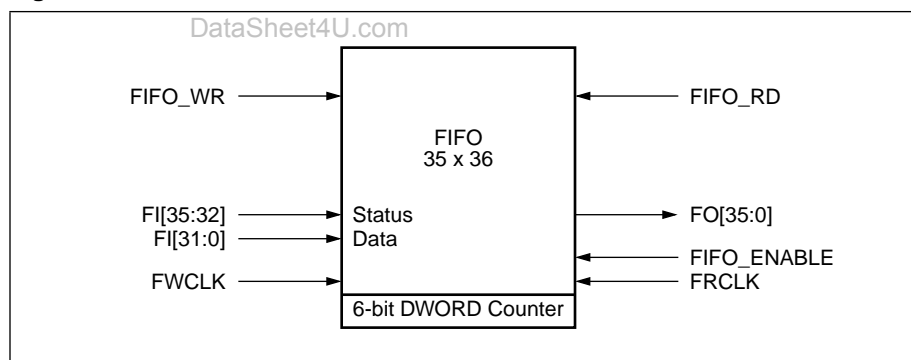
Figure 26. FIFO Interface
