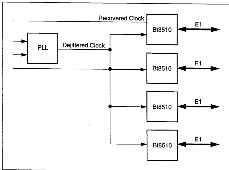
Figure E-1. System Clock Dejittering
