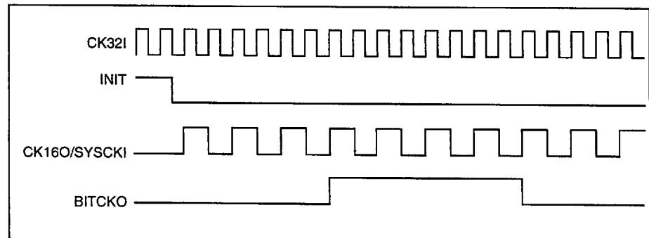
Figure 4. Clock Signals
