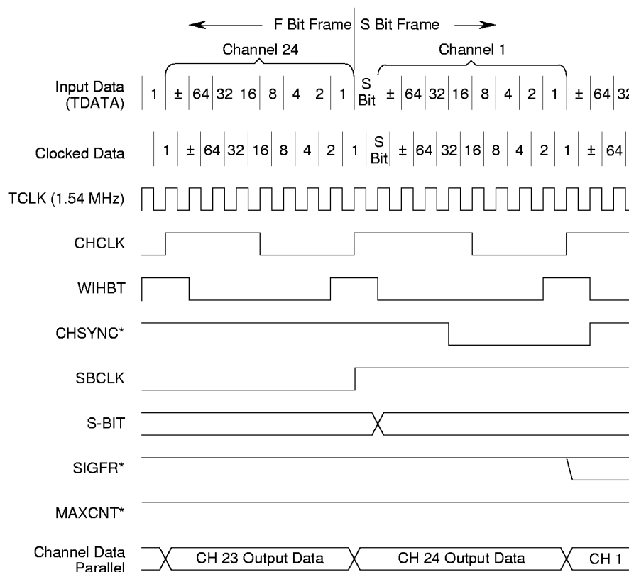
www.DataSheet4U Figure 2. Signal Relationships at Beginning of F_S Frame (S-BIT).
