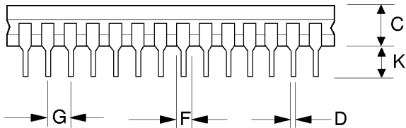
28-Pin Ceramic DIP
