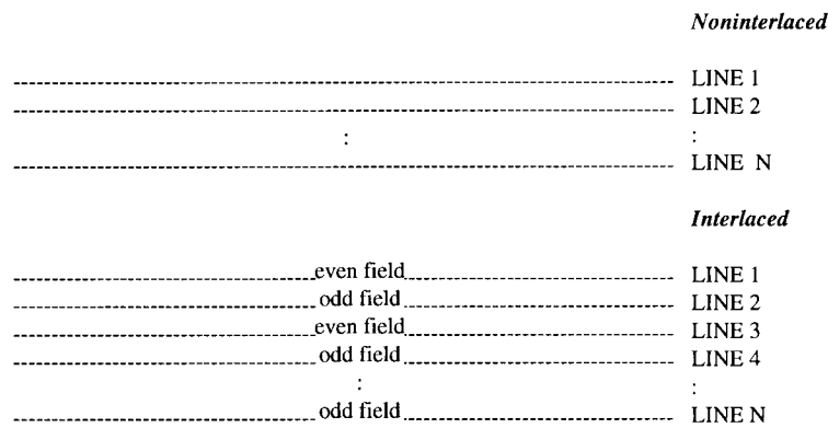
Figure 1. Interlaced / Noninterlaced Display Operation.
