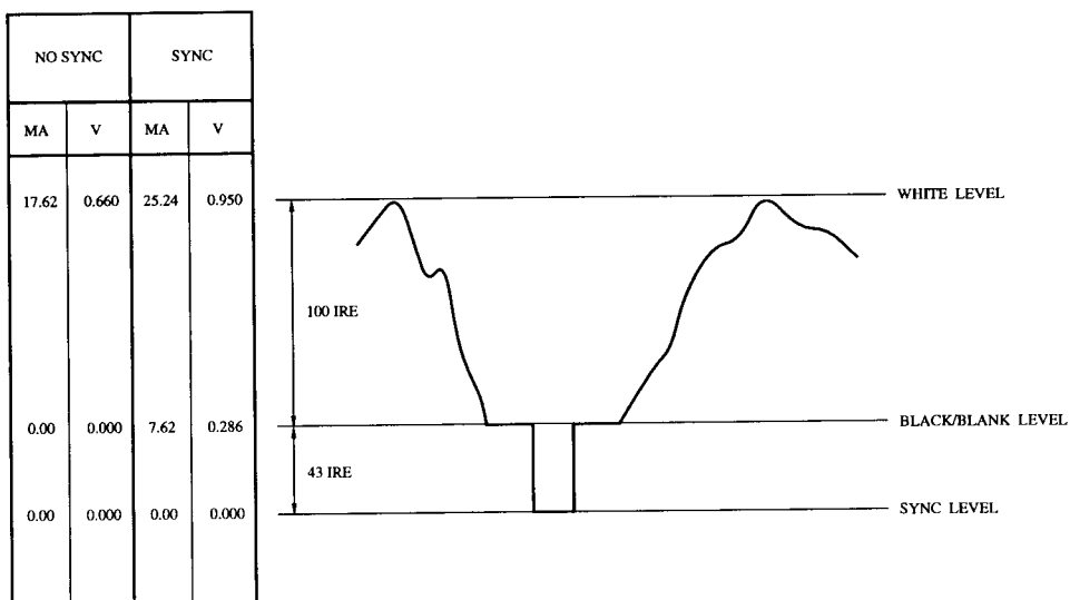
Figure 5. Composite Video Output Waveforms (SETUP = 0 IRE).
