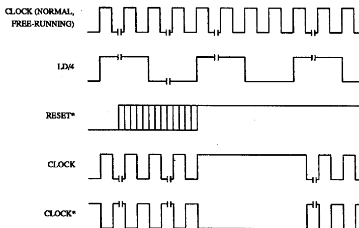
Figure 3. RESET* Timing.
