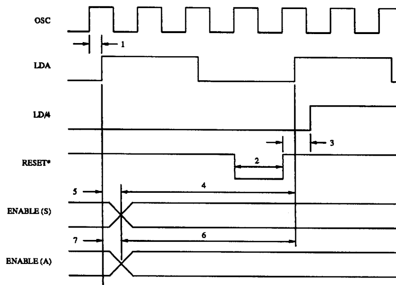
Input/Output Timing
