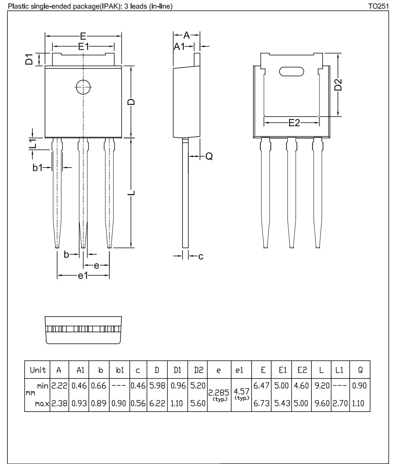
Package Outline IPAK (TO251N)
