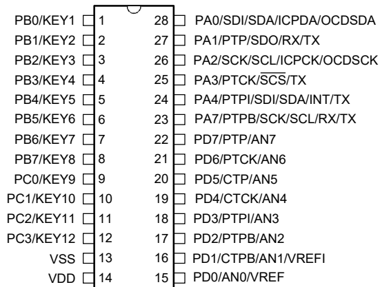
BS84C12CA/BS84CV12CA 28 SOP-A/SSOP-A
