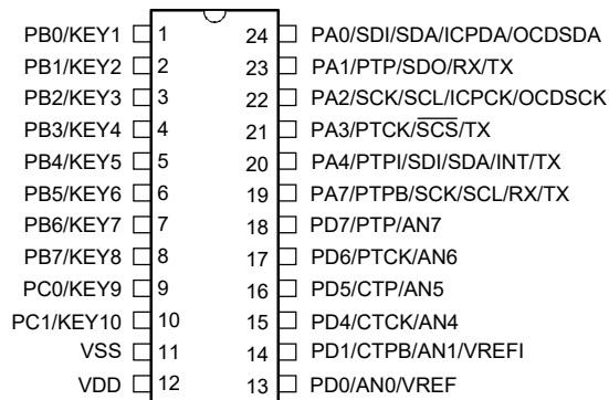
BS84C12CA/BS84CV12CA 24 SOP-A/SSOP-A
