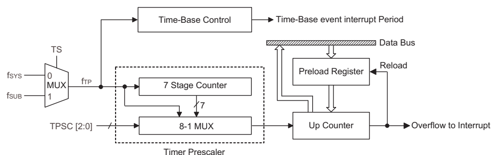
Timer/Event Counter
