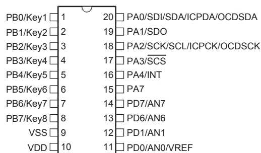
BS84B08A-3/BS84V08A 20 SOP-A/NSOP-A/SSOP-A
