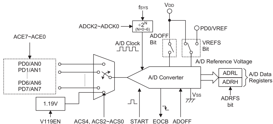
A/D Converter Structure
