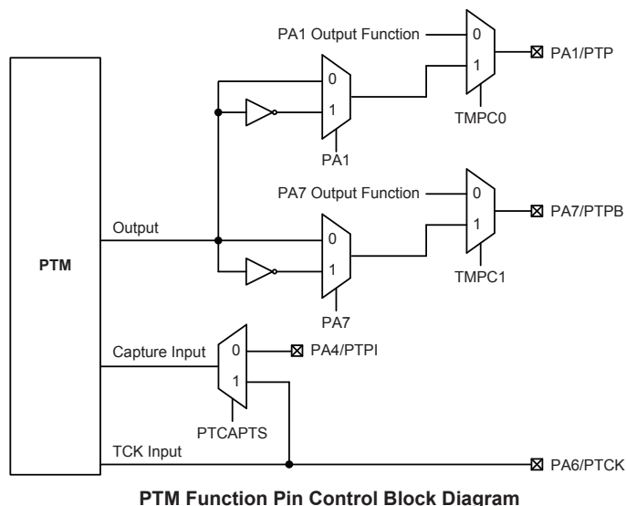
PTM Function Pin Control Block Diagram
