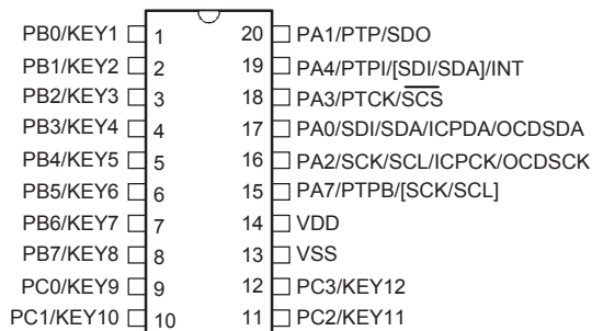
BS83B12C/BS83BV12C 20 SOP-A/SSOP-A
