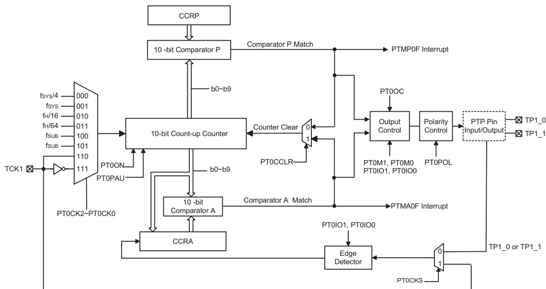
Periodic Type TM Block Diagram
