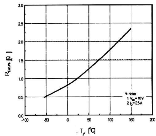
R_{DS(ON)} - T_J
