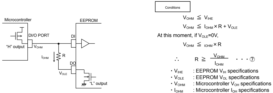
Figure 48. Circuit at DI, DO Direct Connection (Microcontroller DI/O "H" Output, EEPROM "L" output)
