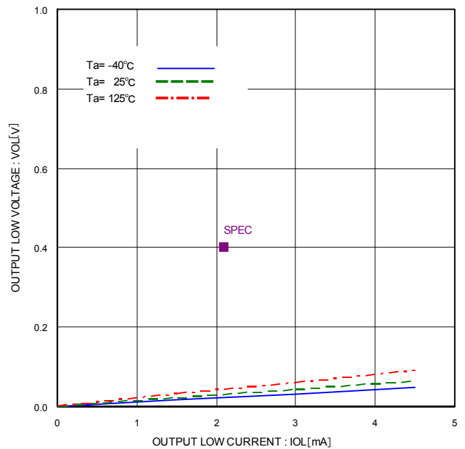
Figure 7. Output Low Voltage vs. Output Low Current ( V_{CC}=4.0\text{V} )
