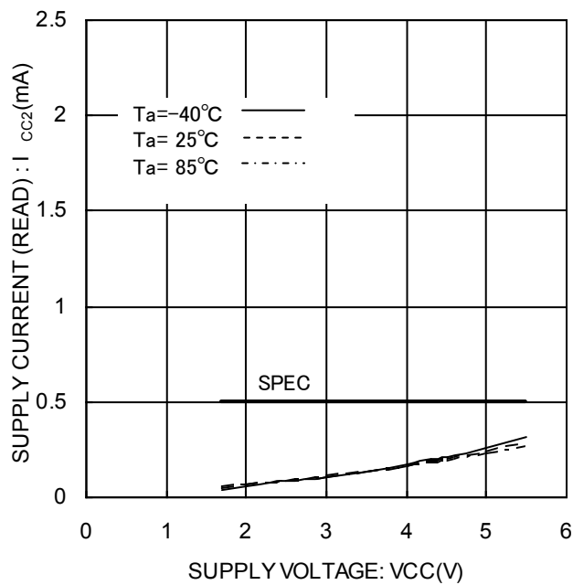
Figure 16 Supply current (READ) I_{cc2}(\text{READ}, f_{sk}=1\text{MHz}) .
