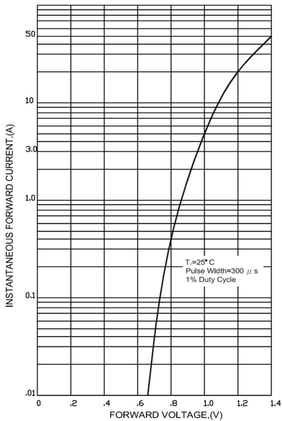
FIG.3-TYPICAL FORWARD CHARACTERISTICS
