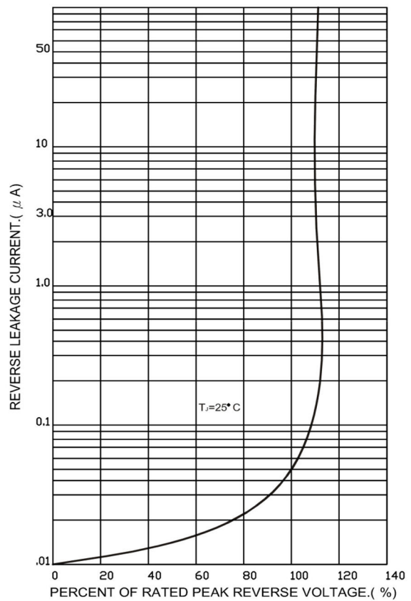
FIG.4-TYPICAL REVERSE CHARACTERISTICS
