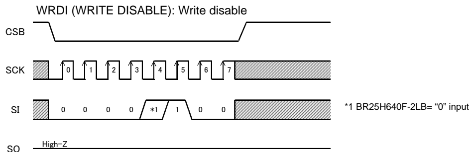
Figure 36. Write disable
