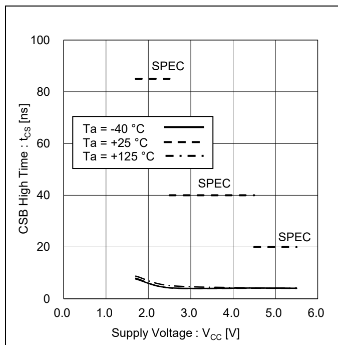
Figure 23. CSB High Time vs Supply Voltage
