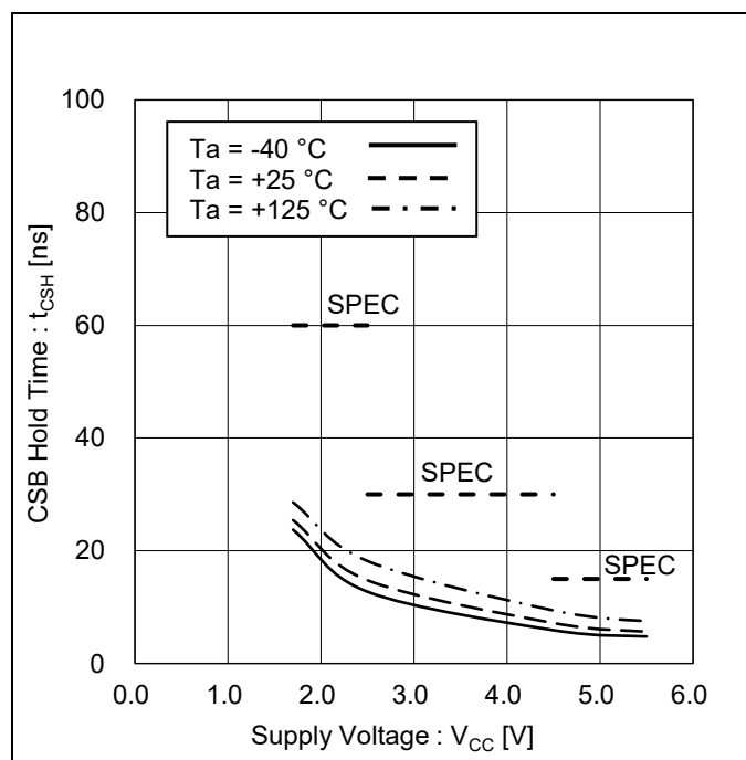
Figure 25. CSB Hold Time vs Supply Voltage
