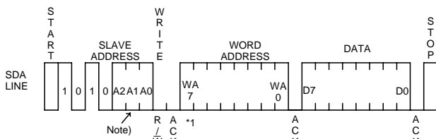
Figure 35. Byte write cycle (BR24L01A/02/04/08/16-W)
