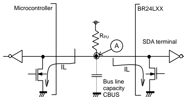
Figure 51. I/O circuit
