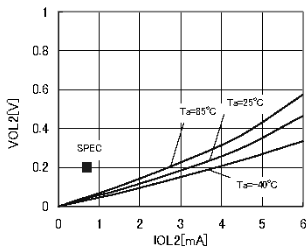
Figure 5. "L" Output Voltage VOL2-IOL2 ( V_{CC}=1.8V )
