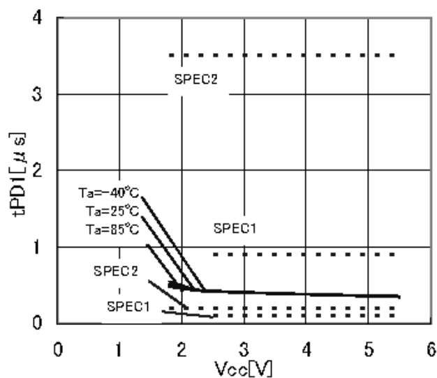
Figure 25. Output data delay time tPD1
