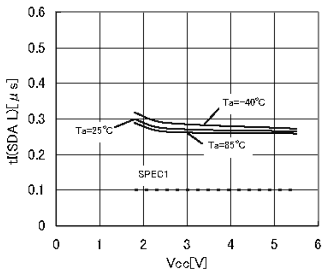
Figure 31. Noise removal valid time t_l(\text{SDA L})
