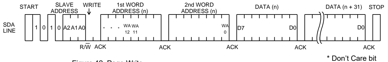
Figure 42. Page Write
