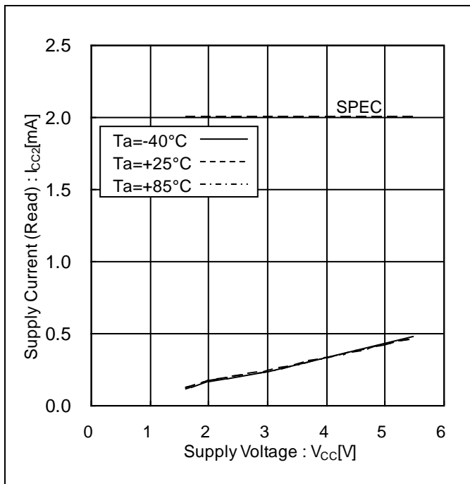
Figure 14. Supply Current (Read) vs Supply Voltage ( f_{\text{scL}}=1\text{MHz} )
