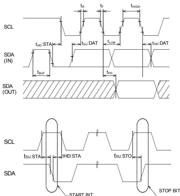
Figure 1. Synchronous Data Timing
