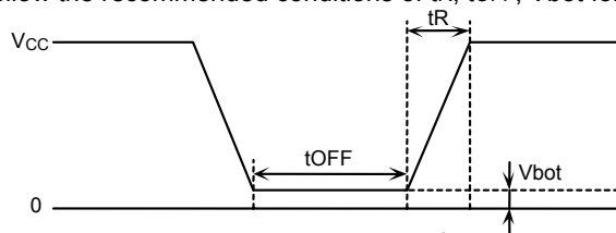
Figure 17. V_{CC} rising wave from 0
