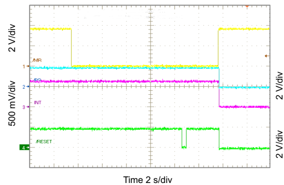
Figure 100. \overline{\text{RESET}} Timing
