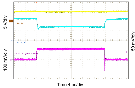
Figure 87. 1.2 V LSLDO Load Transient, 0 to 100 mA
