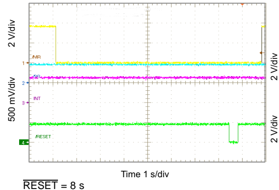
Figure 100. \overline{\text{RESET}} Timing
