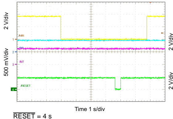
Figure 99. \overline{\text{RESET}} Timing
