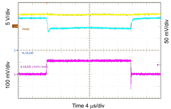
Figure 90. 3.3 V LSLDO Load Transient, 0 to 100 mA
