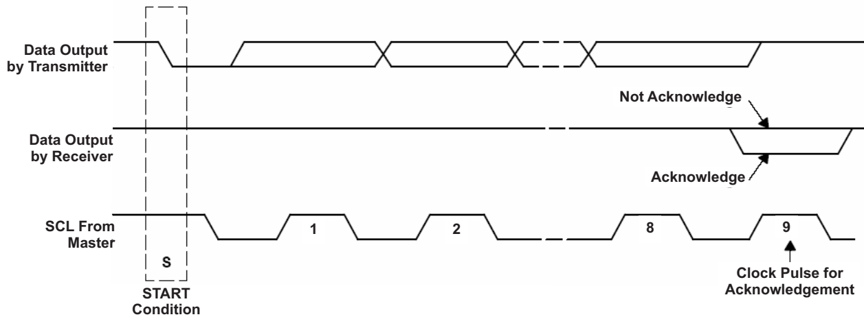
Figure 21. Acknowledge on the I²C Bus
