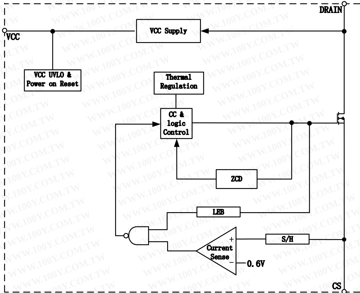
Figure 3. BP9918B Internal Block Diagram
