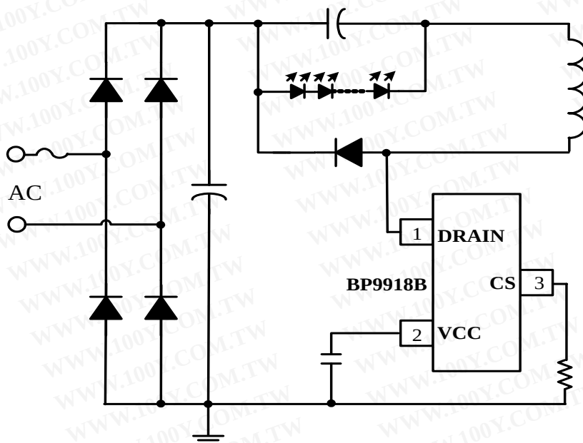
Figure 1. Typical application circuit for BP9918B
