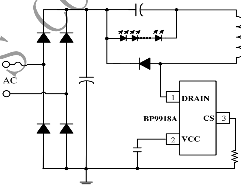
Figure 1. Typical application circuit for BP9918A
