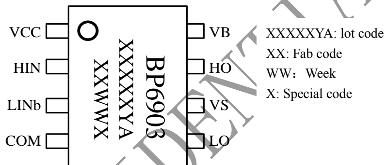
Figure 2. Pin configuration
