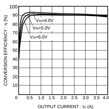
Fig.16 Conversion efficiency
