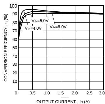
Fig.13 Conversion efficiency
