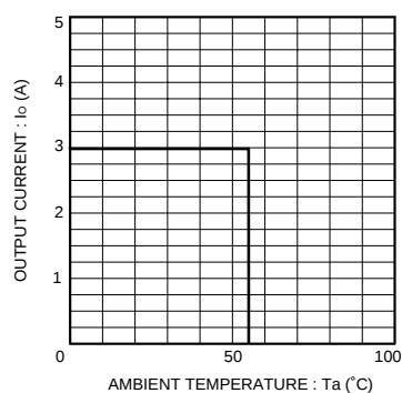
Fig.12 Derating curve
