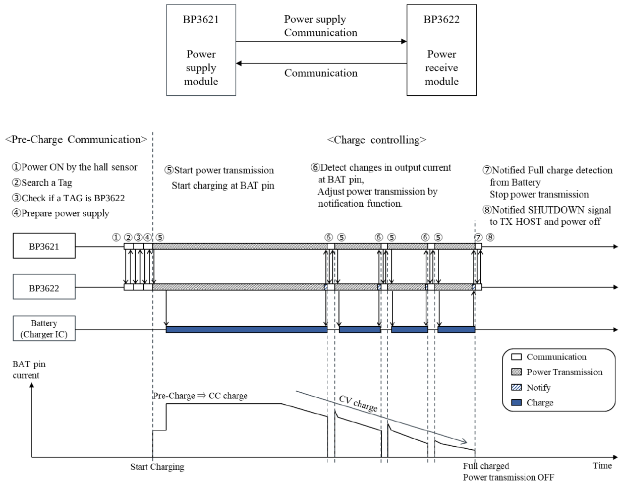
Figure 7. Operation Flow
