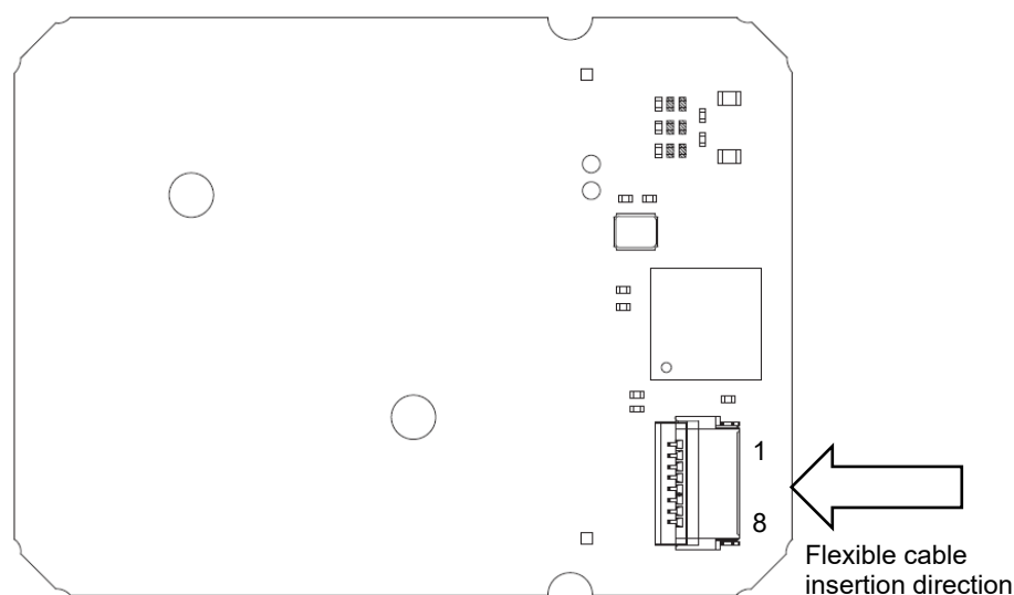
Figure 9. Pin Number (flexible cable connector)
