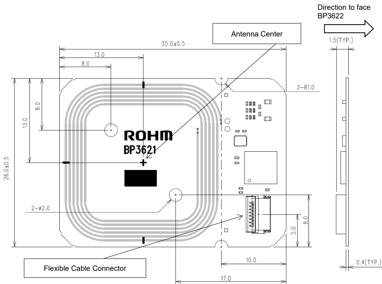
Figure 8. Physical Dimension
