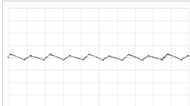
Fundamental output voltage ripple at V_i = 12 V, I_o = 70 A, C_{OUT} = 8 \times 330 \mu F / 10 \text{ m}\Omega + 20 \times 100 \mu F Scale: 10 mV/div, 1 \mu s /div, 20 MHz bandwidth. See section Output Ripple and Noise.
