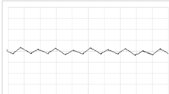
Fundamental output voltage ripple at V_i = 12 V, I_o = 65 A, C_{OUT} = 8 \times 330 \mu F / 10 \text{ m}\Omega + 20 \times 100 \mu F Scale: 10 mV/div, 1 \mu s /div, 20 MHz bandwidth. See section Output Ripple and Noise.
