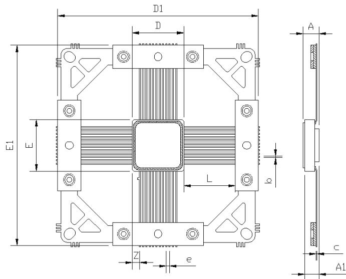
Figure 7-1 CQFP48 package specifications
