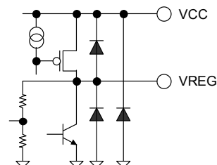
Figure 51. VREG, VCC
