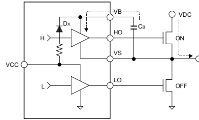
Figure 7. Discharging Period
