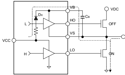
Figure 6. Charging Period
