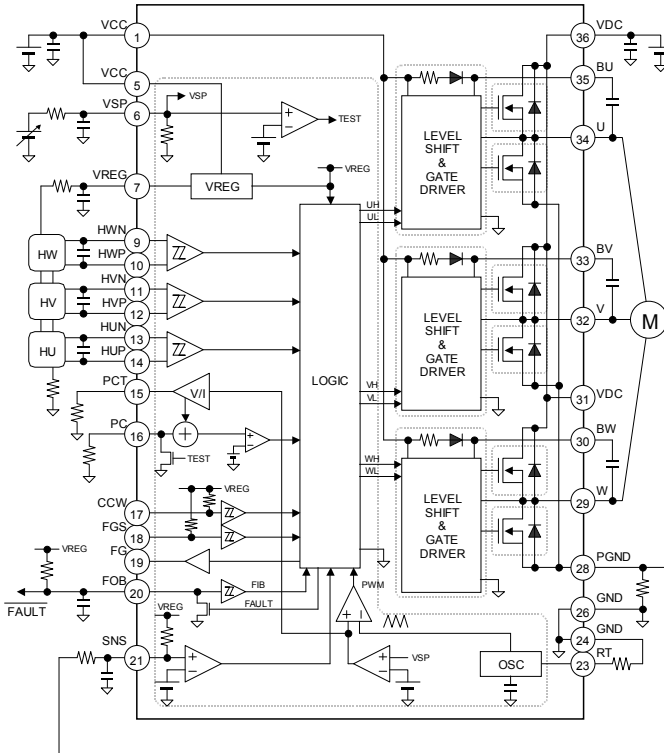
Figure 2. Block Diagram
