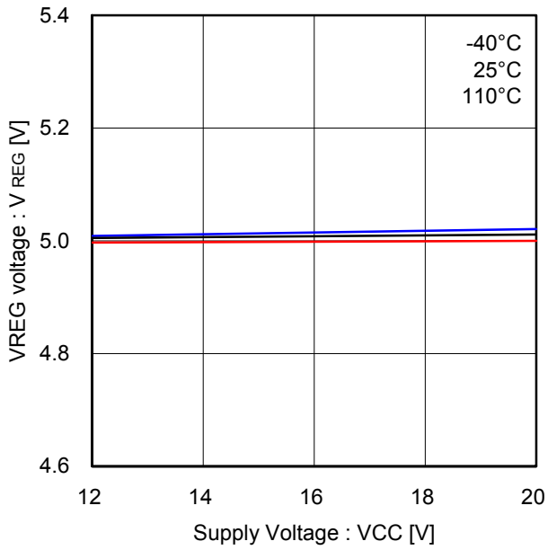
Figure 26. VREG - VCC
