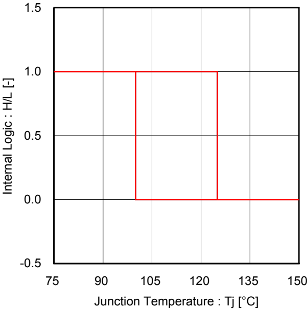
Figure 44. Thermal Shutdown
