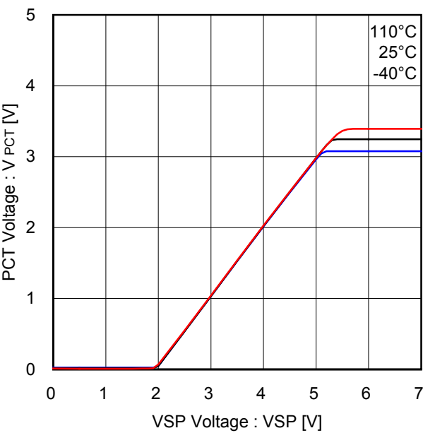
Figure 33. VSP - PCT Offset Voltage
