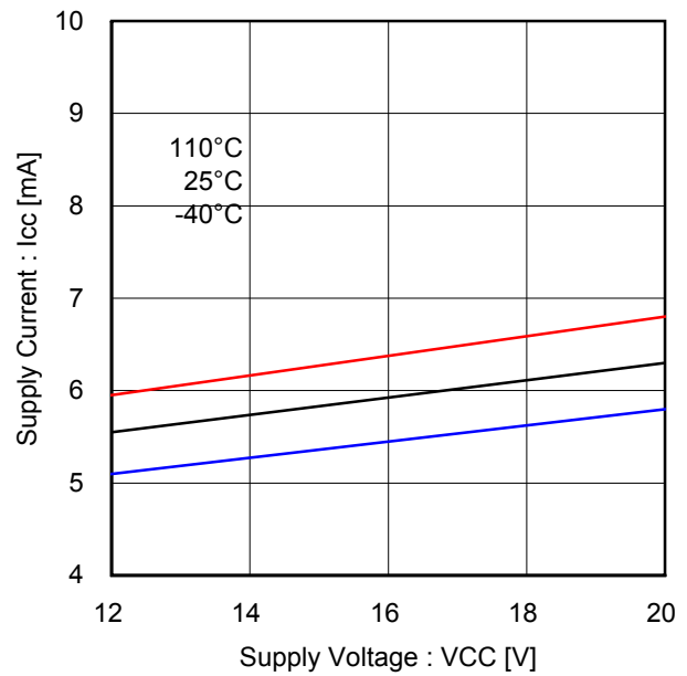
Figure 15. Low Side Drivers Operating Current ( F_{PWM} : 20kHz)
